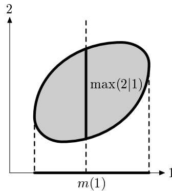
Figure 1: A 2-dimensional set and its characteristics
